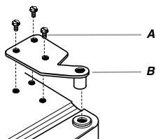
A. \frac{5}{16} " Hex-Head Hinge Screws B. Top Hinge
